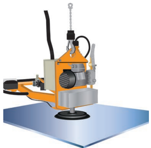
Figure 28 - Ventouse
