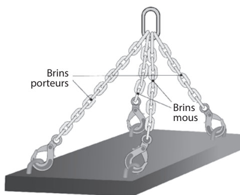
Figure 30 - Élingage charge rigide 4 brins
